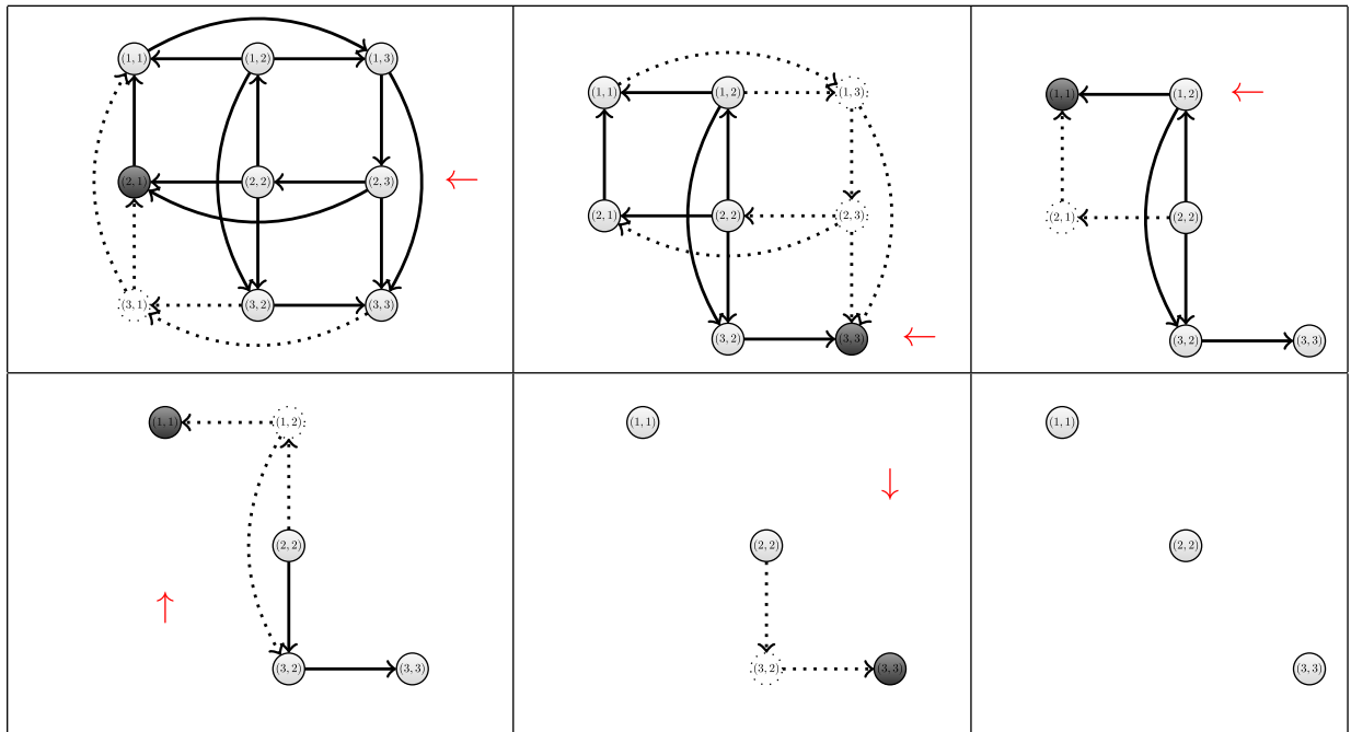
Fig. 3. An illustration of how IDUA R operates.
