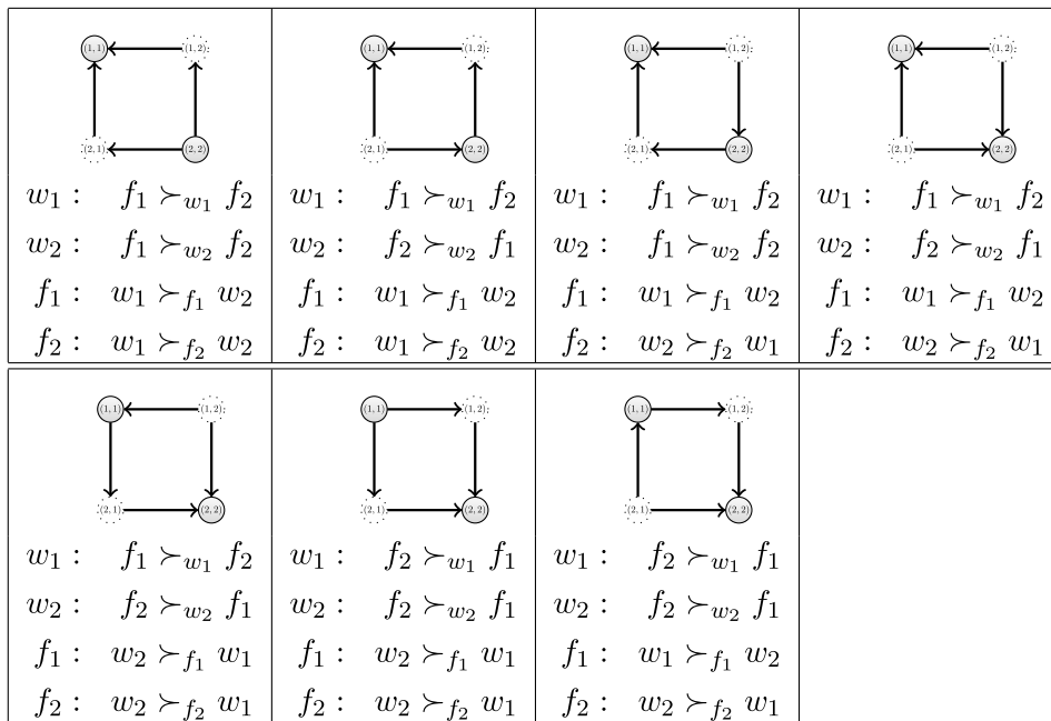
Fig. 4. The 7 instances for which \mu^* is the unique stable matching.
