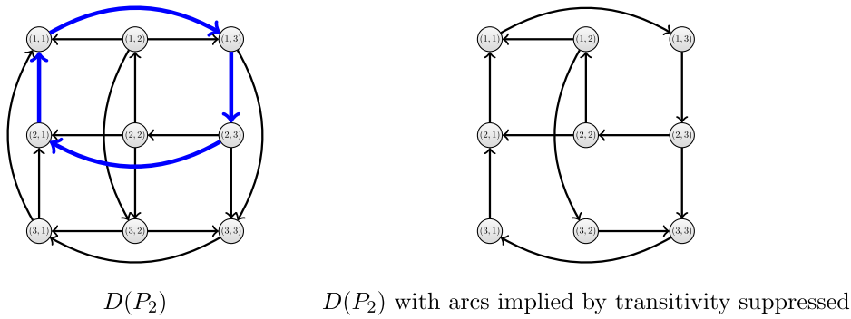
Fig. 2. The matching digraph D(P_2) for the instance P_2 of Example 2. (For interpretation of the colours in the figure(s), the reader is referred to the web version of this article.)
