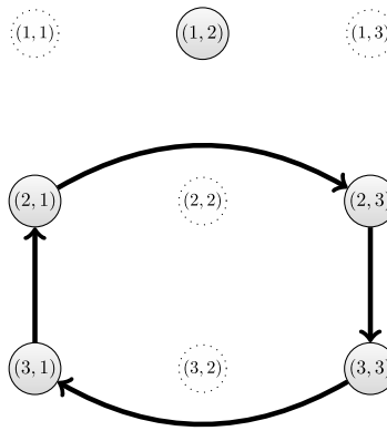
Fig. 1. Illustrating a cycle in the normal form of P_1 from Example 1.
